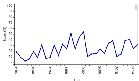
Figure 2. Nitrogen
