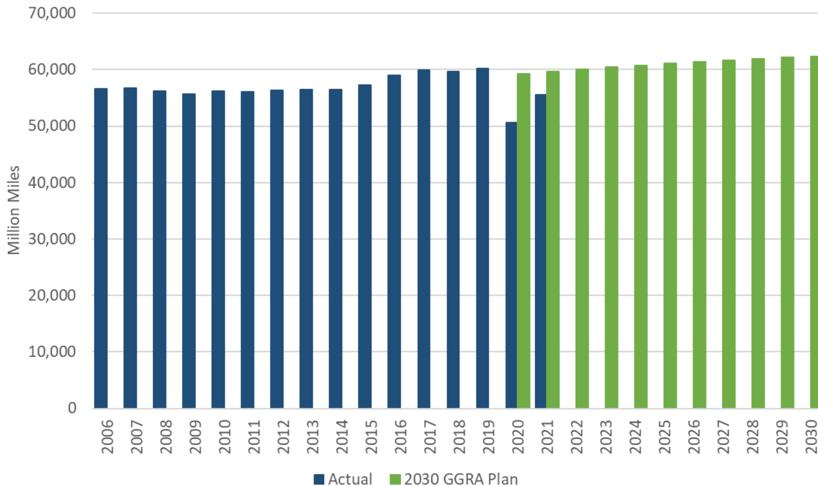
Figure 18. Historic VMT and projected VMT from the 2030 GGRA Plan in millions of miles traveled. (Click figure to return).
