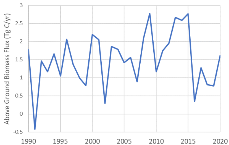
Figure 15. Annual aboveground forest carbon flux in Maryland from the NASA/UMD high resolution forest carbon monitoring product, where positive values represent net growth in the forest carbon sink and negative values (e.g., in 1991) highlight a net loss of carbon due to unfavorable weather conditions and forest disturbance. (Click figure to expand).
