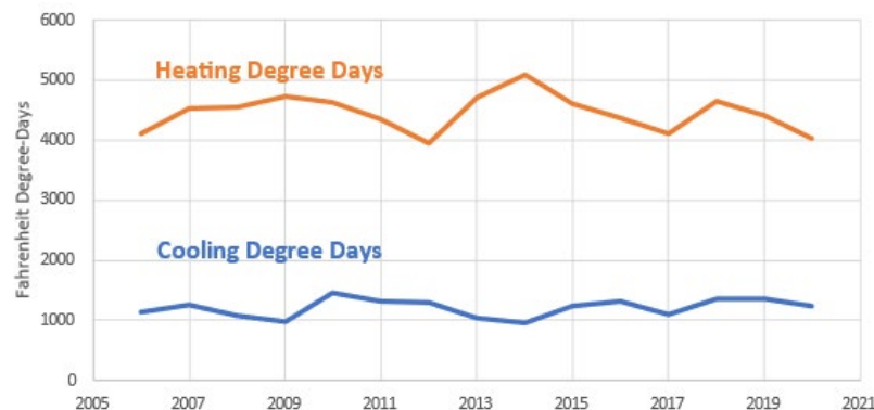
Figure 7. Maryland degree day (NOAA, 2022) s. (Click figure to expand).
