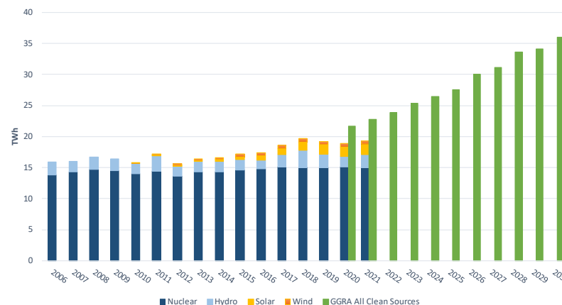
Figure 19. Historic in-state clean and renewable electricity generation as well as projected clean and renewable generation from the 2030 GGRA Plan. (Click figure to expand).
