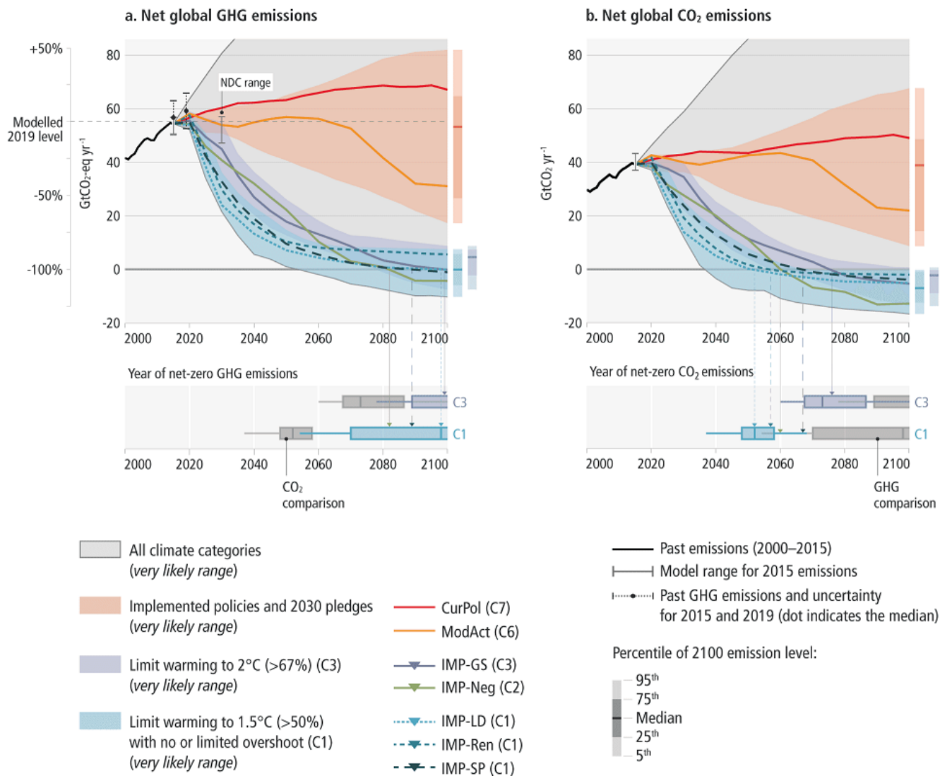
Figure 2. IPCC Working Group III 2.0-degree Celsius and 1.5-degree Celsius pathways. (Click figure to return).
