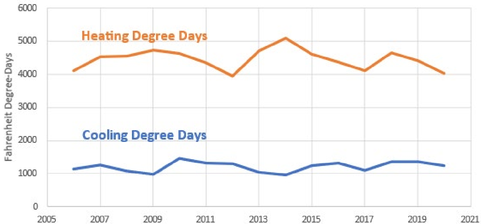
Figure 7. Maryland degree days (NOAA, 2022). (Click figure to return).
