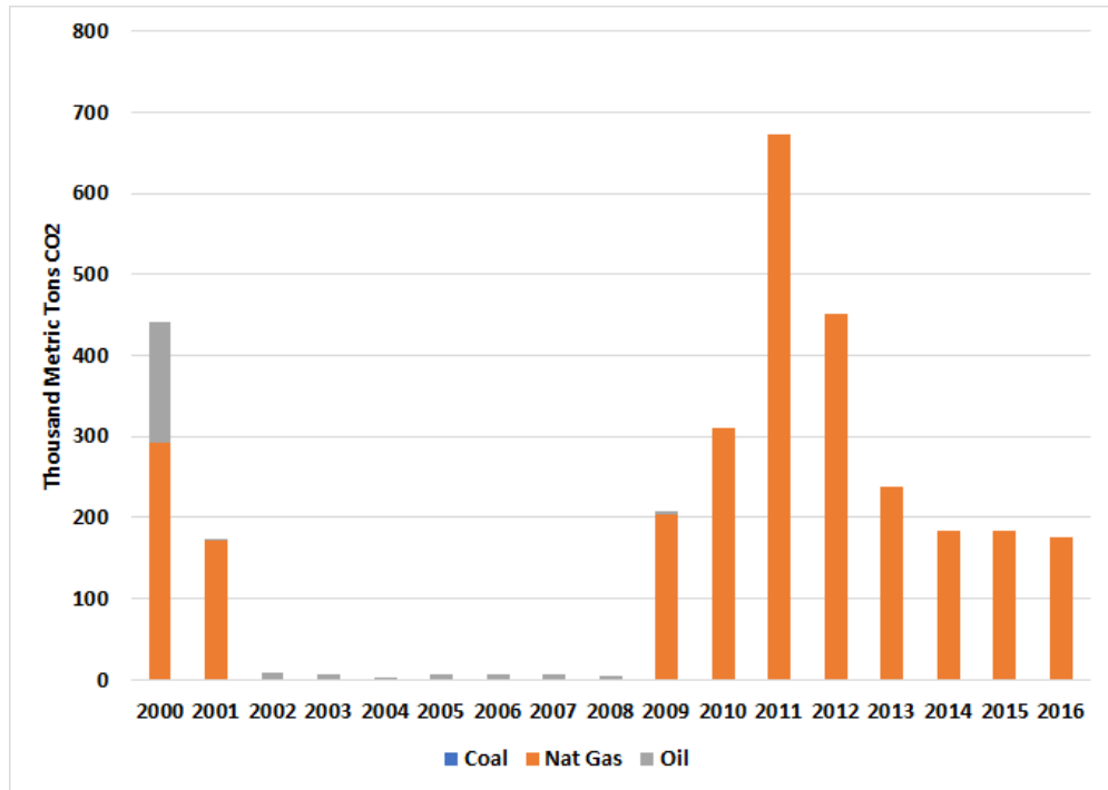
Figure 4-20 Power Sector Carbon Dioxide Emissions by Fuel Source in Slovakia, 2000-2016
