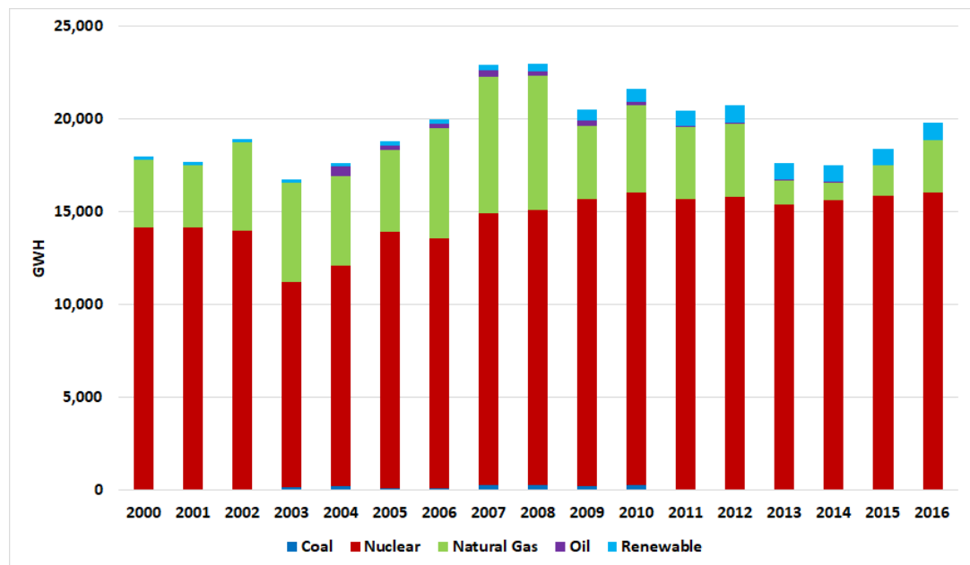
Figure 4-24 Annual Power Generation by Source in Hungary, 2000-2016
