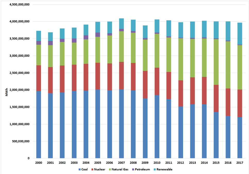
Figure 4-3 U.S. Power Generation by Source, 2000-2016 73
