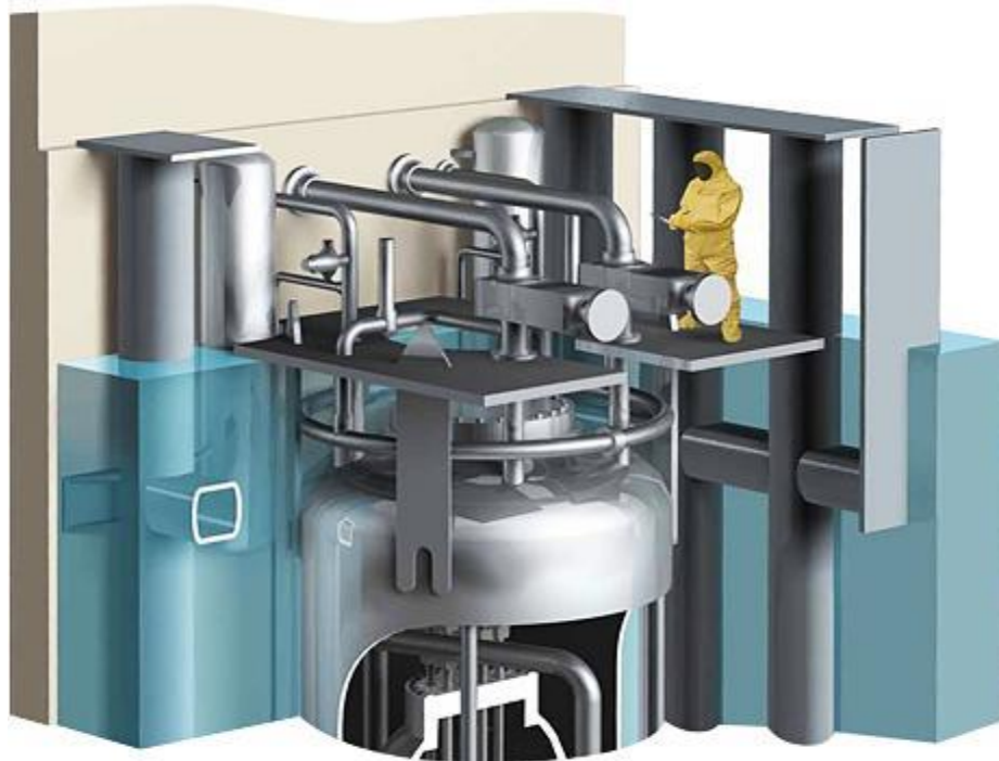
Figure 3-1 NuScale Power Module
