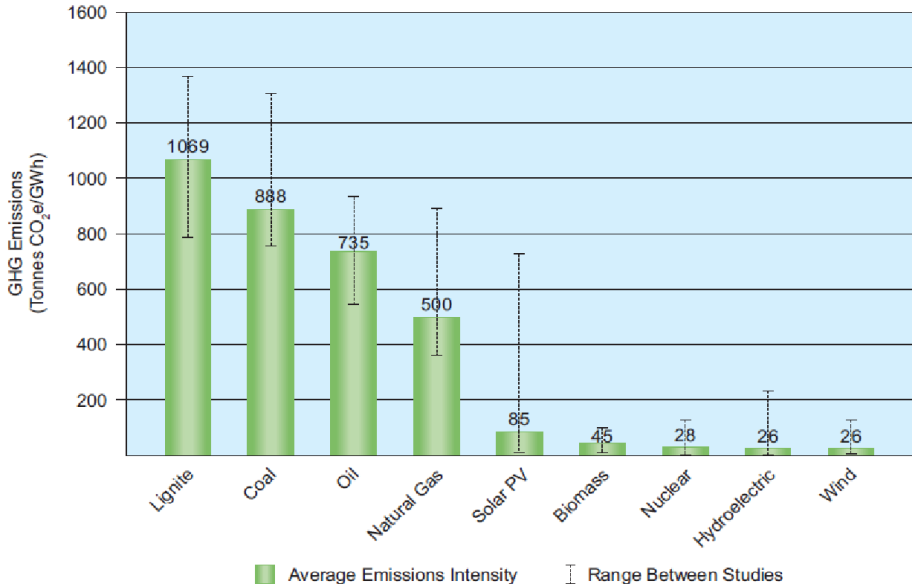
Figure 2-1 Lifecycle GHG Emissions of Various Electricity Generation Methods
