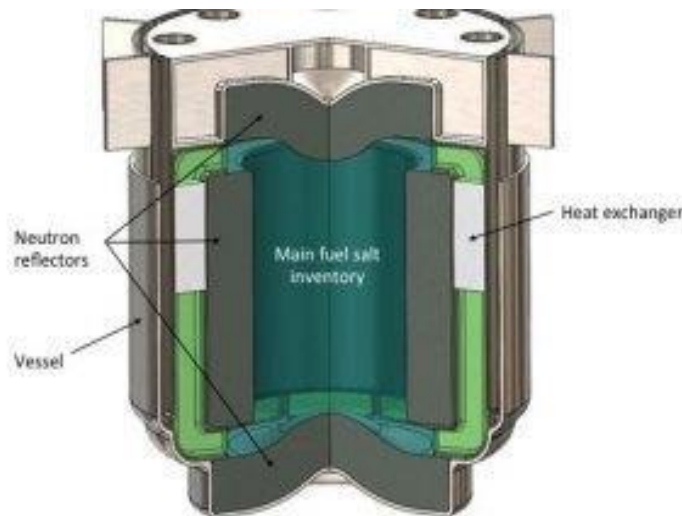
Figure 3-8 A Traveling Wave Reactor
