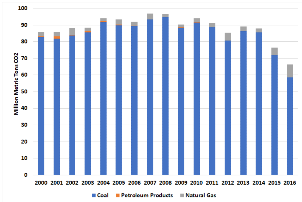
Figure 4-7 Power Sector Carbon Dioxide Emissions by Fuel Source, South Carolina, 2000- 2016
