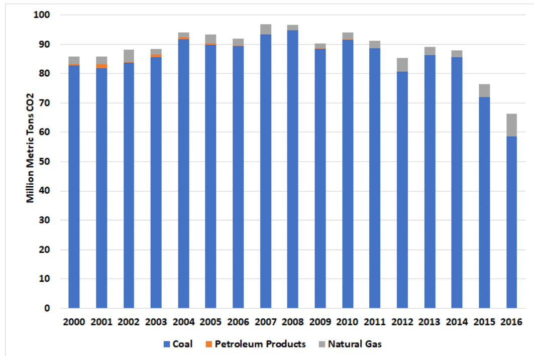
Figure 4-10 Power Sector Carbon Dioxide Emissions by Fuel Source, Illinois, 2000-2016
