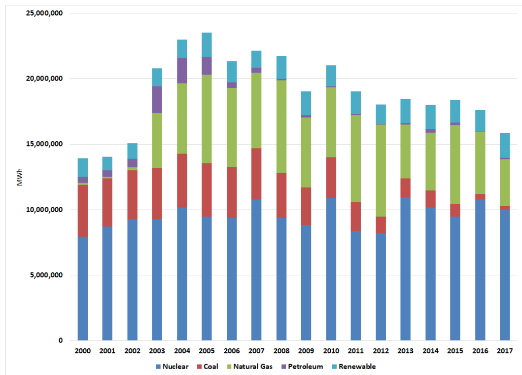
Figure 4-11 Annual Power Generation by Source in New Hampshire, 2000-2017
