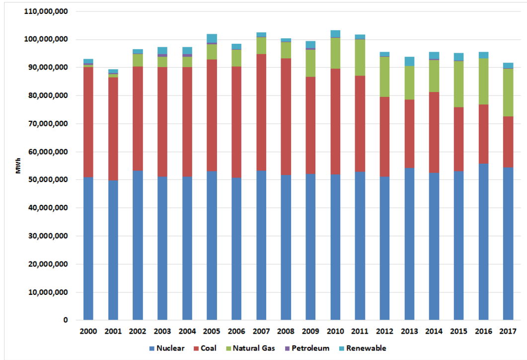
Figure 4-5 Annual Power Generation by Source in South Carolina, 2000-2017
