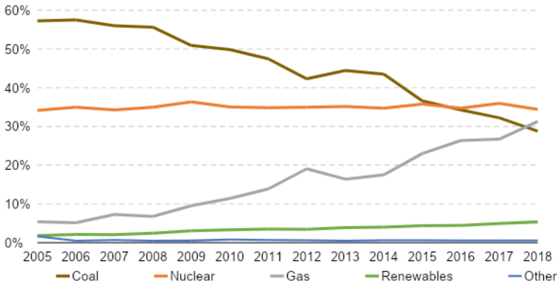
Figure 1-3 Share of PJM Generation (in GWh), by Fuel Source (2005-2018)
