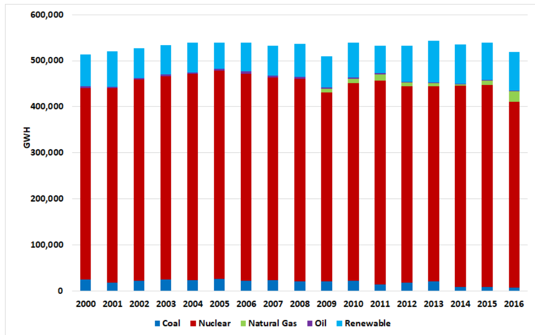
Figure 4-15 Annual Power Generation by Source in France, 2000-2016
