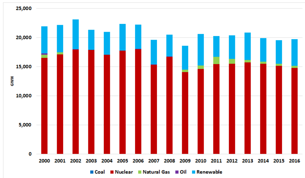
Figure 4-18 Annual Power Generation by Source in Slovakia, 2000-2016
