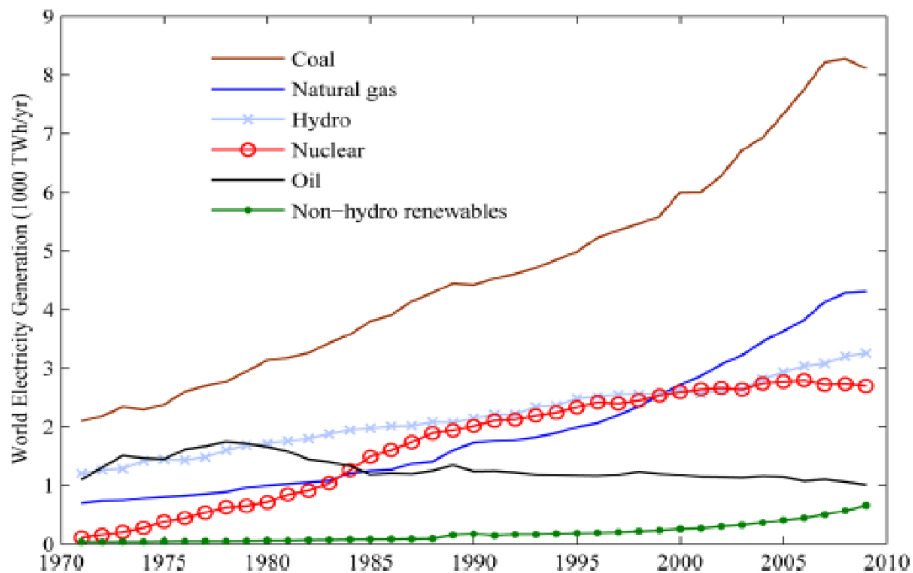
Figure 2-3 World Electricity by Electrical Power Source for the Historical Period 1971- 2009
