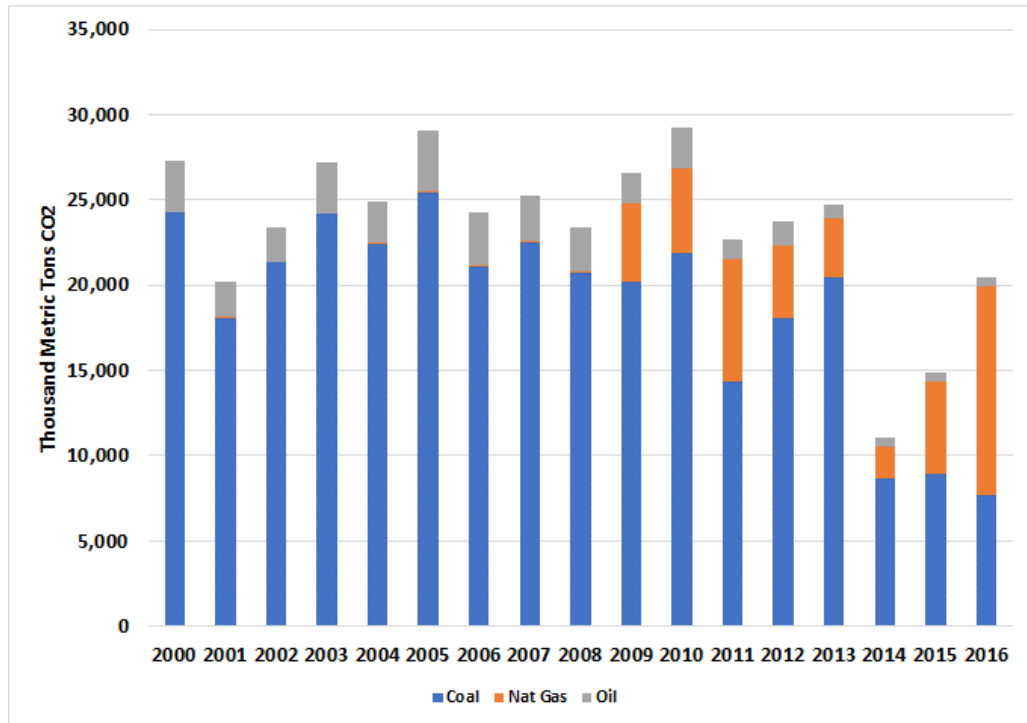
Figure 4-17 Power Sector Carbon Dioxide Emissions by Fuel Source in France, 2000-2016
