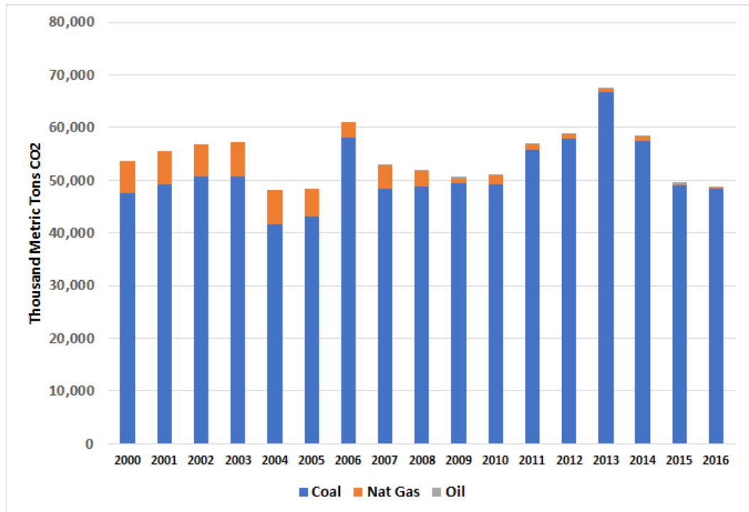
Figure 4-23 Power Sector Carbon Dioxide Emissions by Fuel Source in Ukraine, 2000-2016
