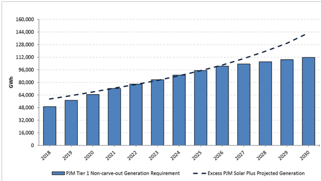
Figure III-2. Non-carve-out Tier 1 RPS Requirements in PJM Compared to Projected Available PJM Renewable Energy Generation (2018-2030)
